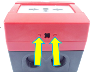
Pic. 7 - To remove the front activation element push the two locking hooks at the bottom of the call point; use the two pins located at the side of the supplied call point's reset key.
