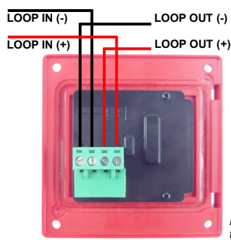
Pic. 3 - Insert the supplied pluggable terminal block connector to the socket positioned on the back of the loop interface plate.
