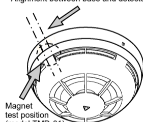
Picture 5 - The correctly installed detector.
